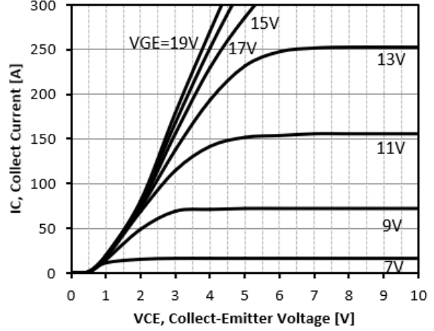
Figure 6: Typical IGBT Output characteristics, T_J=150^{\circ}\text{C}; t_p=300\mu\text{s}
