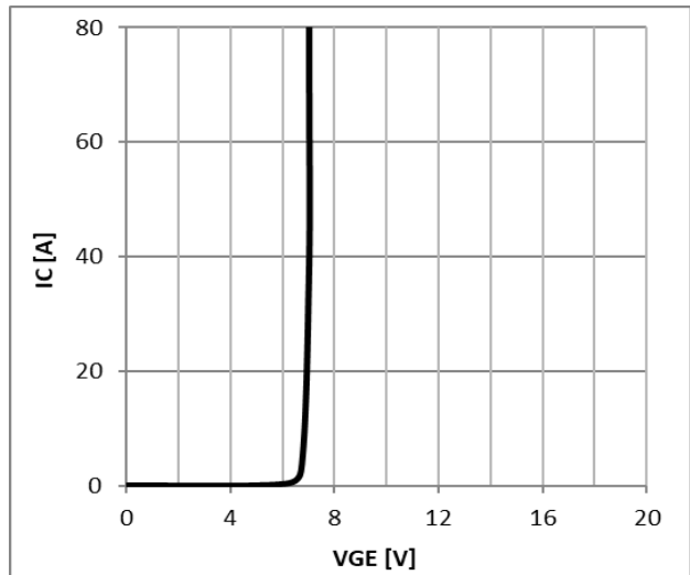
Figure 4: Typical Gate Threshold Voltage
