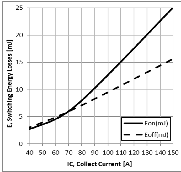
Figure 9: Typical Energy Loss VS. IC, TC=25°C, L=200uH, VCE=600V, VGE=15V, RG=15 Ω
