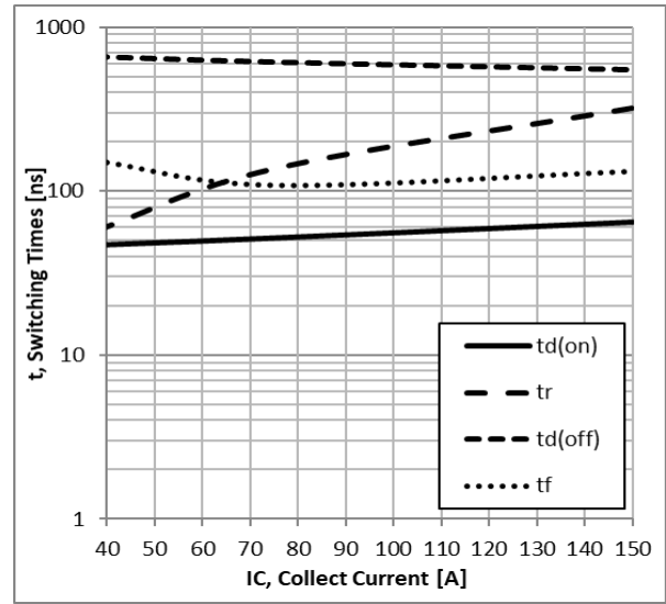
Figure 10: Typical Switching Time VS. IC, TC=25°C, L=200uH, VCE=600V, VGE=15V, RG=15 Ω
