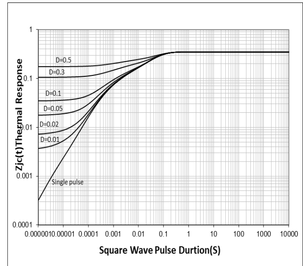
Figure 12: Normalized transient thermal impedance junction-to-case
