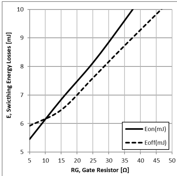
Figure 7: Typical Energy Loss VS. R_G , T_C=25^{\circ}\text{C} , L=200\mu\text{H}, V_{CE}=600\text{V}, V_{GE}=15\text{V}, I_C=75\text{A}
