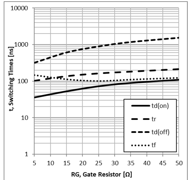
Figure 8: Typical Switching Time VS. R_G , T_C=25^{\circ}\text{C} , L=200\mu\text{H}, V_{CE}=600\text{V}, V_{GE}=15\text{V}, I_C=75\text{A}
