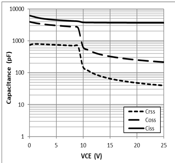
Figure 11: Typical Capacitance VS. VCE, VGE=0V, f=1MHz
