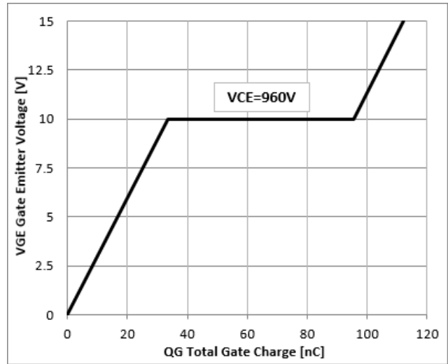
Figure 4: Typical Gate charge VS. VGE, IC=25A
