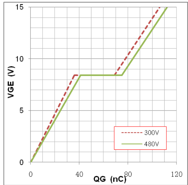
Figure18:typical gate charge VS. VGE,IC=30
