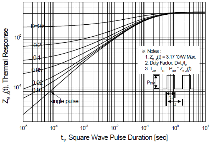
Figure 11-2. Transient Thermal Response Curve for JFFC10N65C
