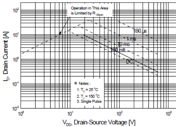
Figure 9-1. Maximum Safe Operating Area for JFPC10N65C
