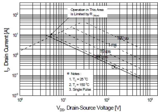
Figure 9-2. Maximum Safe Operating Area for JFFC10N65C
