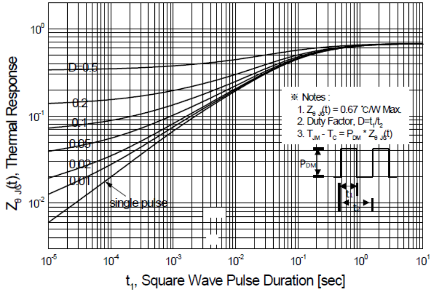
Figure 11-1. Transient Thermal Response Curve for JFPC10N65C
